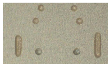
Dots 0.011" (0.27 mm) of structural and electrical conductive adhesives dispensed by Time Pressure Liquid Dispensing Pump
